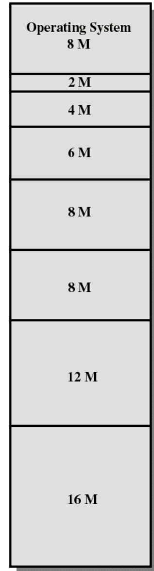
Unequal-size partitions
