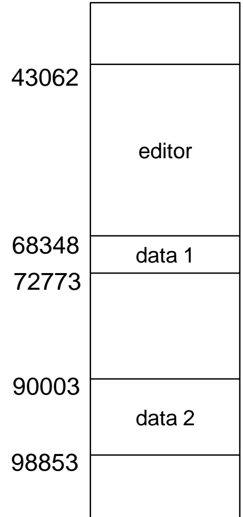
physical memory
